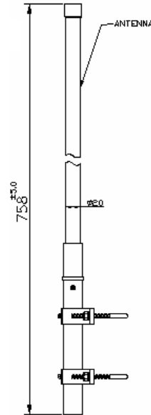
Antenna + mount
